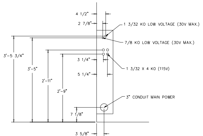
DETAIL "A"
